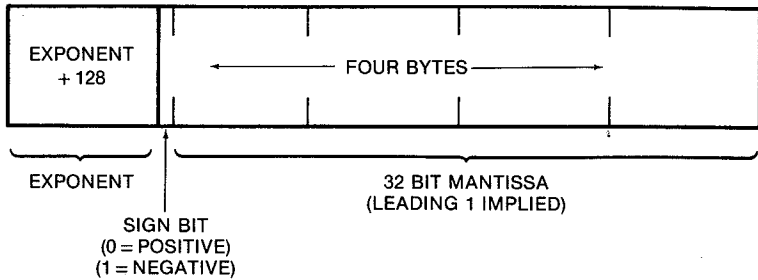
Fig. 3-3. Data structure for floating point value.
